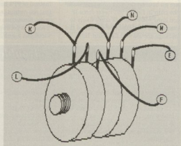
Figure 3: The volume control
