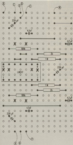
Figure 1: Vero board layout – the copper tracks run vertically. X indicates a cut in the track
