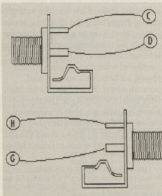
Figure V: The speaker outputs – 3.5mm jack sockets
